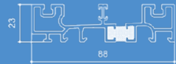
Patio Low Threshold (Silver or Gold) 104324
