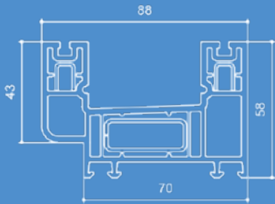
58mm Outer Frame 105178 Steel U Channel 113018 Steel Box 713104 (S51104)
