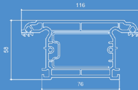
Patio Midrail 705252 (P58252) Steel Channel 713166 (S00166)
