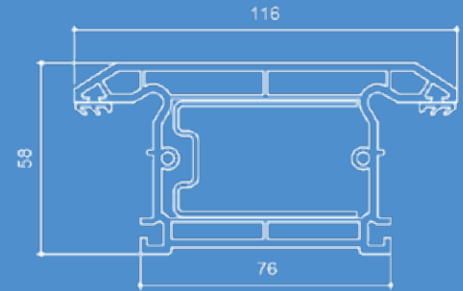
Patio Midrail 702152 (P58152) Steel Channel 713166 (S00166)
