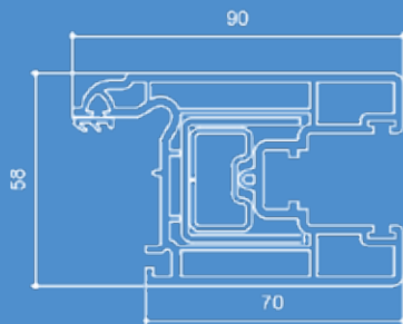
Patio Sash 703251 (P58251) Steel Channel 713029 (S00029) *Steel Channel (Prep'd) 713804 (S00127) Steel Box(400mm) 713119 (S00119) Steel Box (4000mm) 713124 (S00124)
